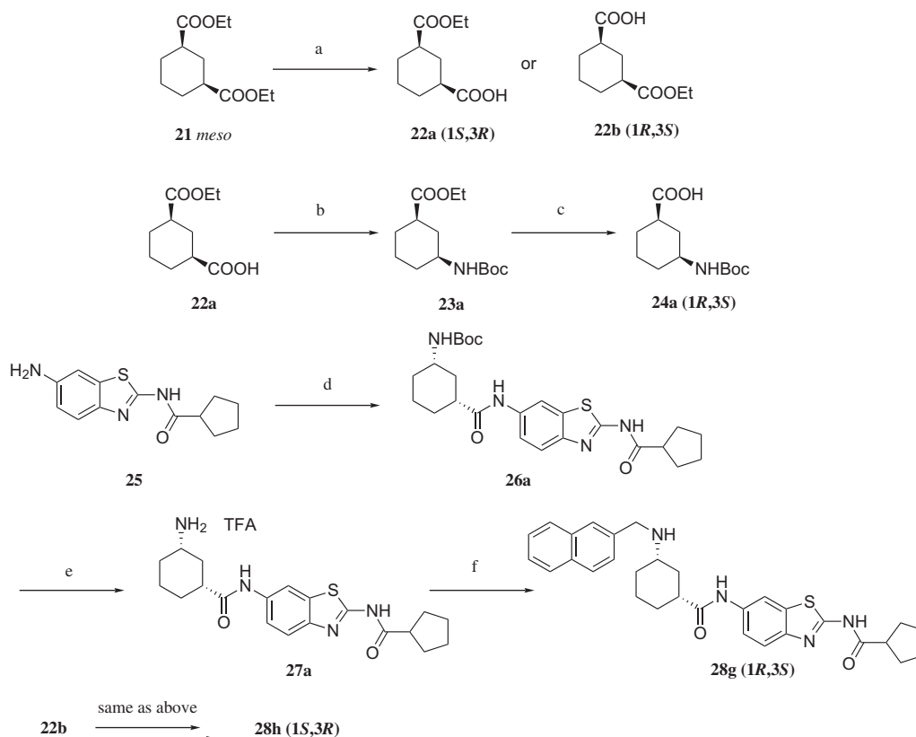
Scheme 4. (a) Lipase AYS Amano for 22a or Lipase PS Amano for 22b , pH 7.2 phosphate buffer; (b) (PhO) 2 PON 3 , Et 3 N, toluene, then t -BuOH; (c) 5 N-NaOH, THF; (d) 24a , EDC, HOBt, DMF; (e) TFA, CH 2 Cl 2 ; (f) 2-naphthaldehyde, MP-BH(OAc) 3 , DMF.
