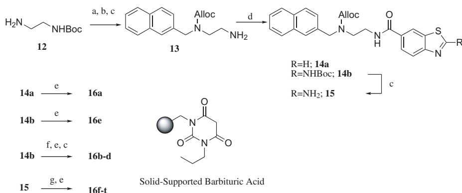
Scheme 2. Reagents and conditions: (a) 2-naphthaldehyde, NaBH(OAc) 3 , DCE; (b) Alloc-Cl, K 2 CO 3 , THF–H 2 O; (c) 50% TFA–CH 2 Cl 2 ; (d) benzothiazole-6-carboxylic acid for 14a , 2- N -Boc-aminobenzothiazole-6-carboxylic acid for 14b , EDC, HOBT, DMF; (e) solid-supported barbituric acid, Pd(PPh 3 ) 4 , THF; (f) Aryl CH 2 Br or Alkyl CH 2 Br, K 2 CO 3 , DMF; (g) Ac 2 O, DMAP, CH 2 Cl 2 , or carboxylic acid, EDC, HOBT, DMF.
