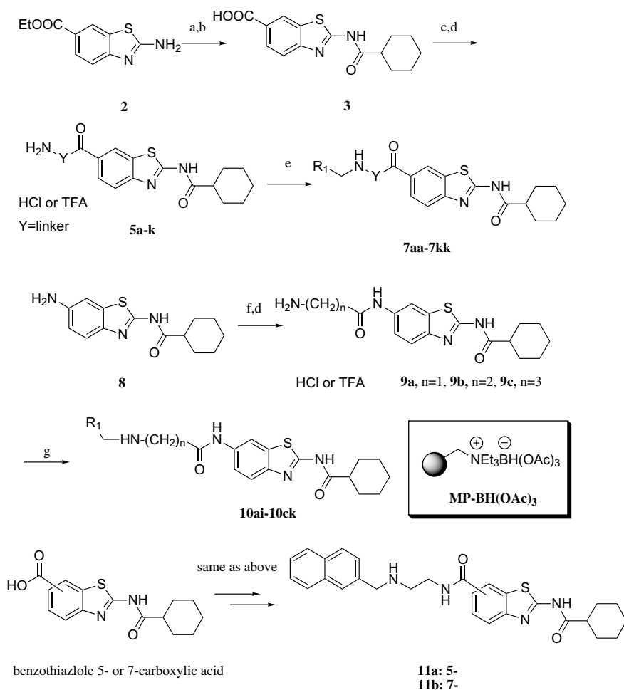
Scheme 1. Reagents and conditions: (a) cyclohexanecarboxylic acid, EDC, HOBT, DMF; (b) 1 N-NaOH, MeOH; (c) BocNH-linker-NHR ( 4a–k ), EDC, HOBT, DMF; (d) 4 N-HCl/dioxane or 50% TFA-CH 2 Cl 2 ; (e) R 1 CHO ( 6a–k ), MP-BH(OAc) 3 , DMF, then PS-CHO, catch and release purification using MP-TsOH then 2 M-NH 3 /MeOH; (f) BocNH(CH 2 ) n COOH, EDC, HOBT, DMF; (g) R 1 CHO ( 6i–k ), MP-BH(OAc) 3 , DMF.
