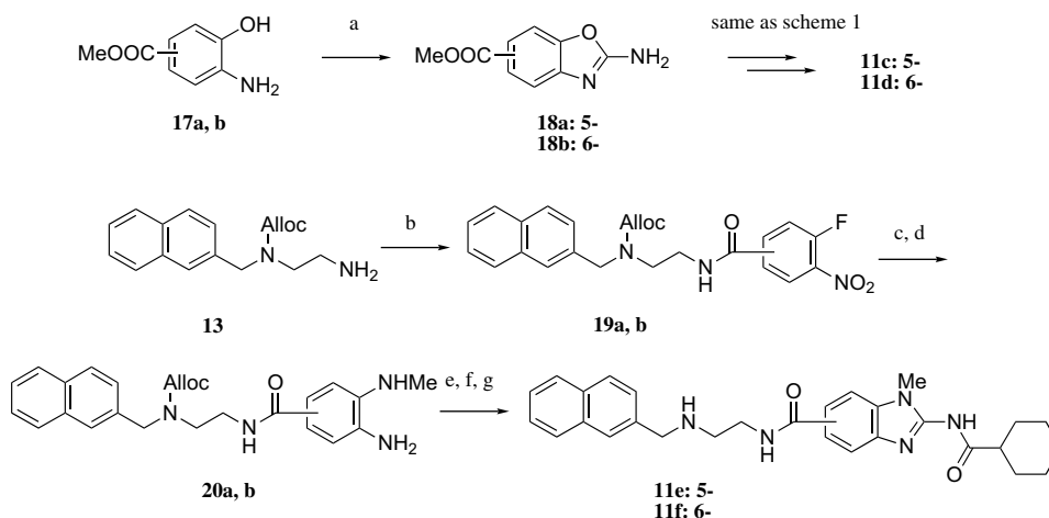
Scheme 3. Reagents and conditions: (a) di-(imidazole-1-yl) methanimine, THF; (b) 4-fluoro-3-nitrobenzoic acid for 19a , 3-fluoro-4-nitrobenzoic acid for 19b , EDC, HOBt, DMF; (c) MeNH 2 –THF; (d) SnCl 2 ·2H 2 O, 6 N-HCl, EtOH; (e) cyclohexanecarbonyl isothiocyanate, CH 2 Cl 2 ; (f) EDC, DIEA, CH 2 Cl 2 ; (g) solid-supported barbituric acid, Pd(PPh 3 ) 4 , THF.
